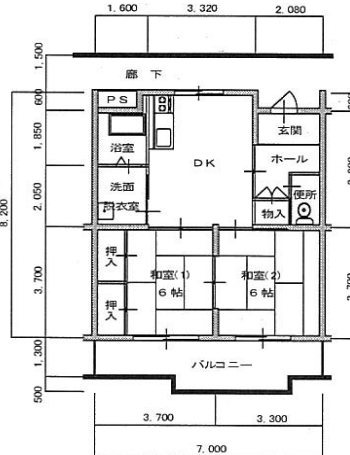
C・D棟 (2DK)
